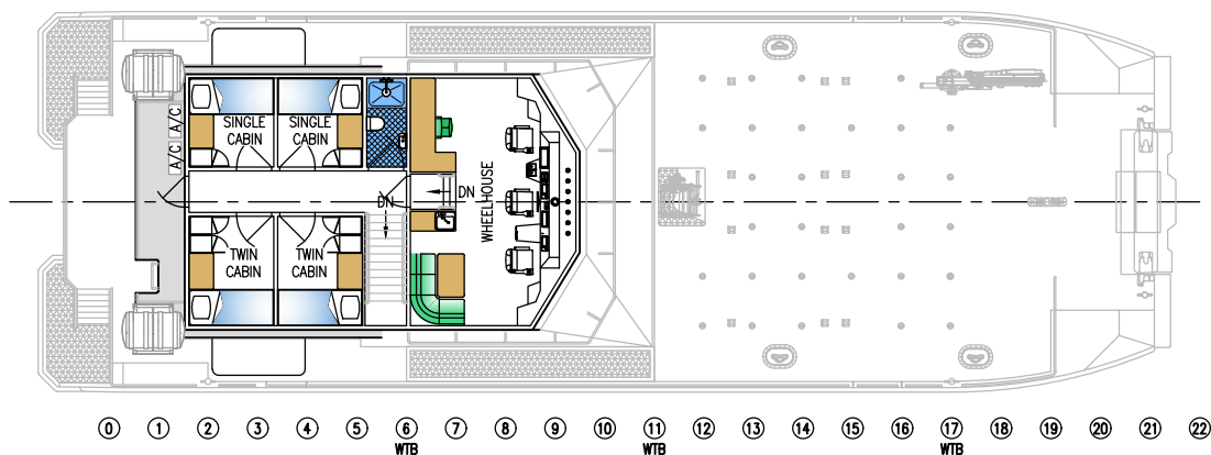
UPPER DECK
