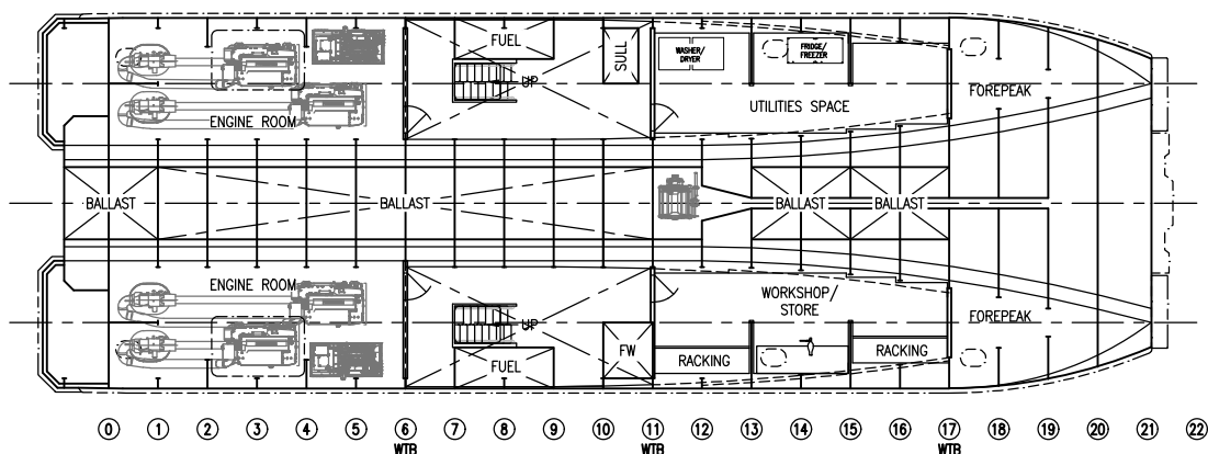
HULL PLAN
