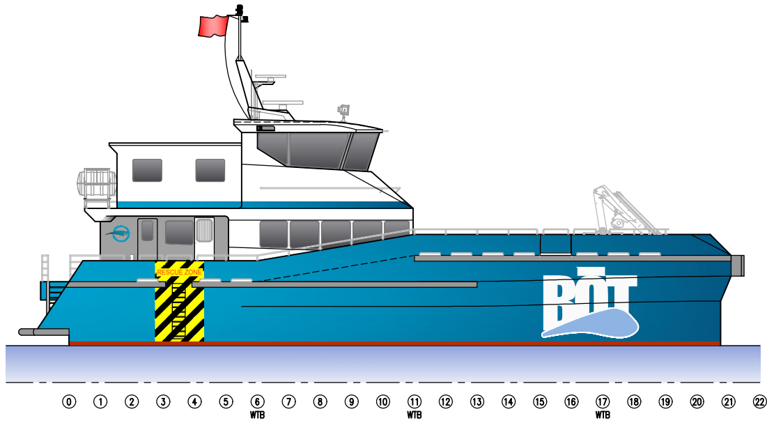
OUTBOARD PROFILE
