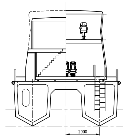
TYPICAL SECTION
