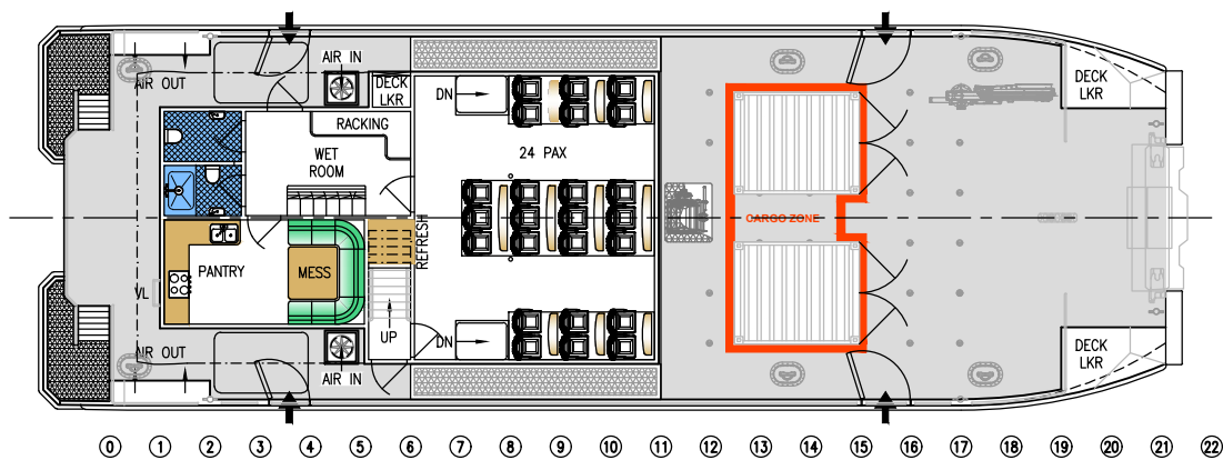
MAIN DECK
