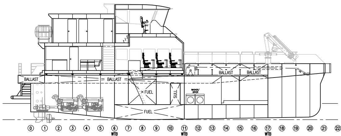
INTERNAL PROFILE
